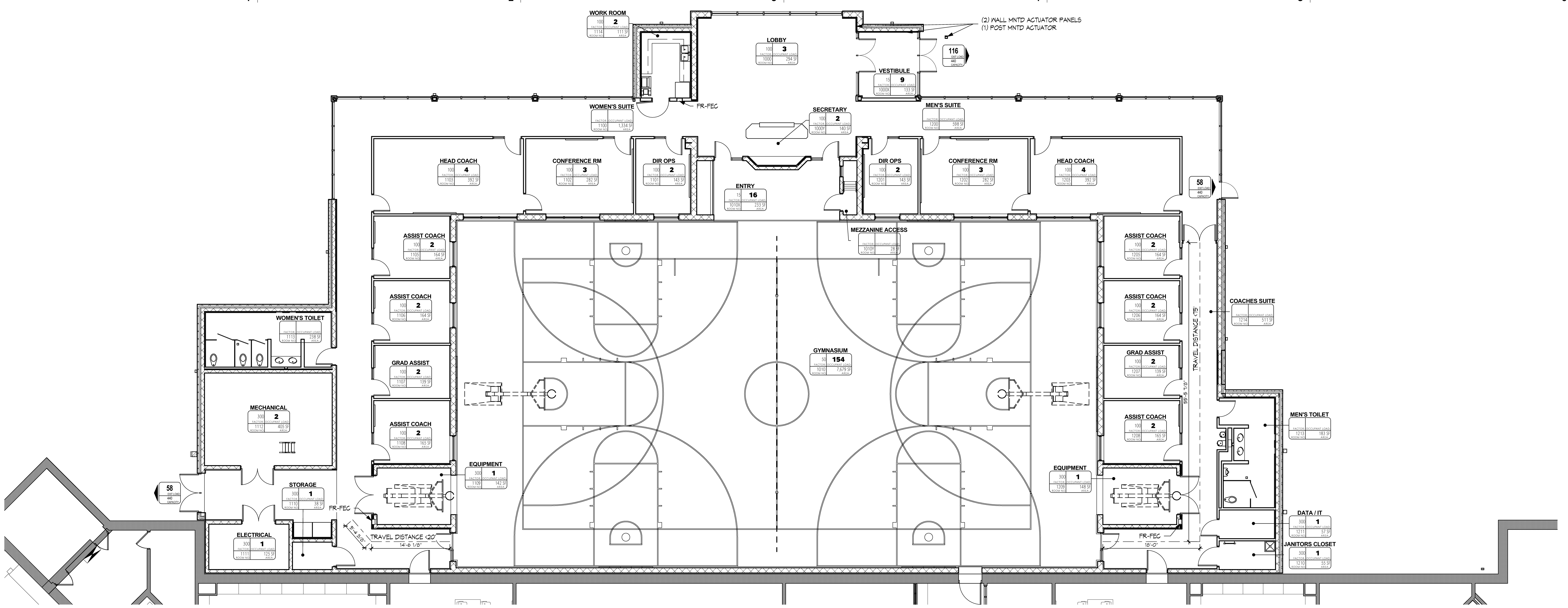
C LOWER LEVEL CODE PLAN SCALE | 1/8" = 1'-0"
