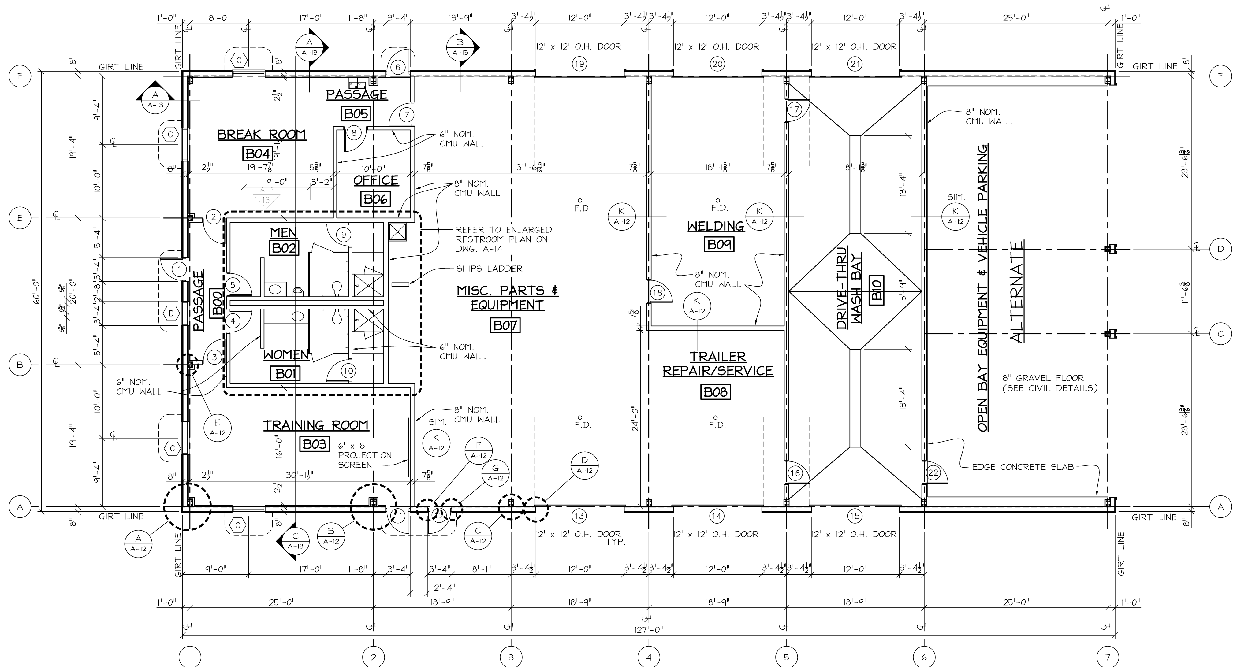
FLOOR PLAN - BUILDING "B" SCALE: 1/8"=1'-0"
