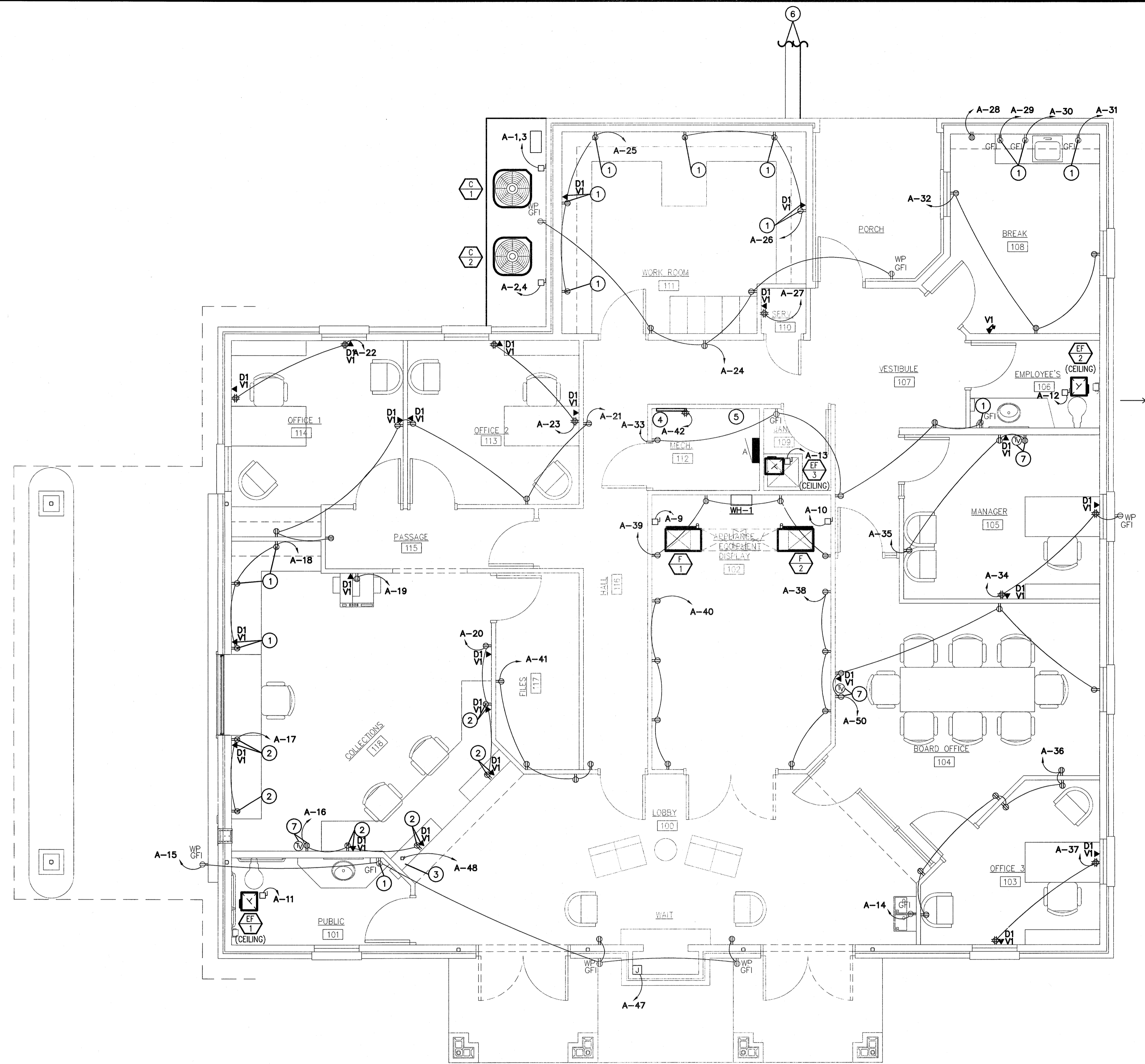
PLAN NORTH FLOOR PLAN SCALE: 1/4" = 1'-0"
